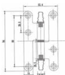
Pernios de acero para puerta interior con remate Steel hinge for interior door with crown tip
