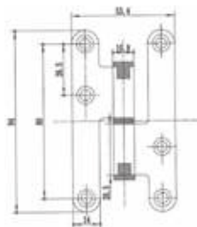
Pernios de acero para puerta interior sin remate Steel hinge for interior door with flat tip
